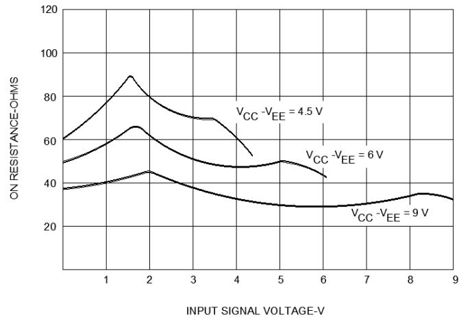
TYPICAL ON RESISTANCE VS INPUT SIGNAL VOLTAGE
