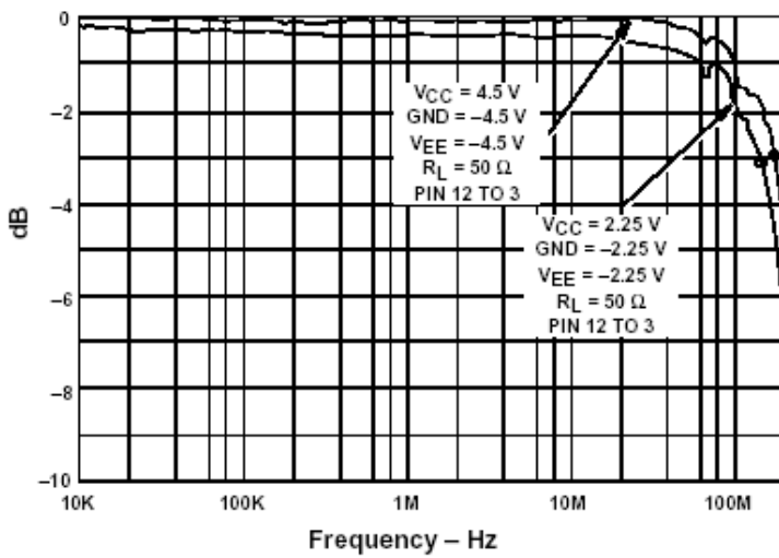
CHANNEL ON BANDWIDTH
