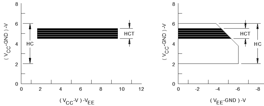
FIGURE 1. Recommended operating area as a function of supply voltages.
