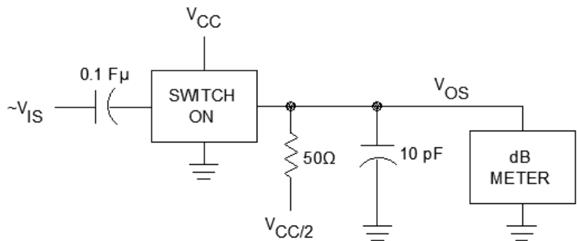
FREQUENCY-RESPONSE TEST CIRCUIT
