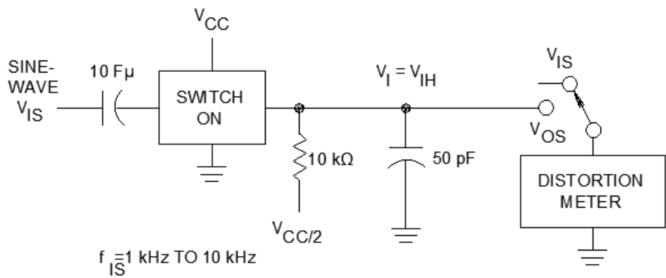
SINE-WAVE DISTORTION TEST CIRCUIT
