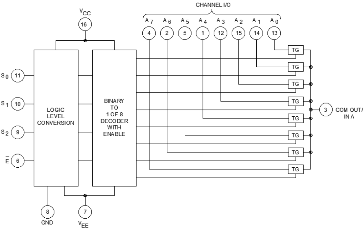
FIGURE 4. Logic diagram.
