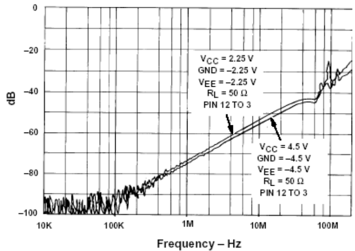
CHANNEL OFF FEED THROUGH
