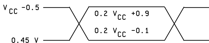
AC TESTING: INPUT, OUTPUT WAVEFORMS
