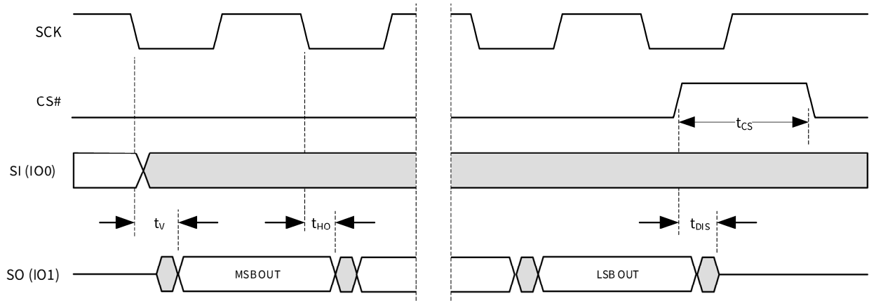
SPI single bit output timing
