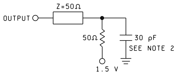
CIRCUIT A
