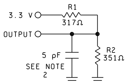
CIRCUIT B
