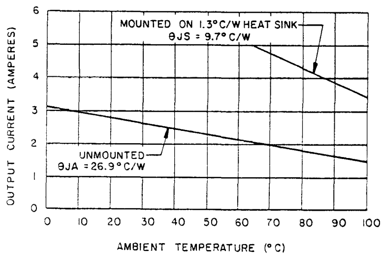
FIGURE 5. Output current vs ambient temperature.
