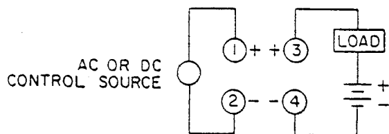
CIRCUIT DIAGRAM TERMINAL VIEW
