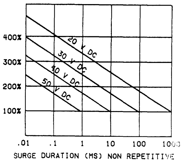
FIGURE 5. Maximum allowable overloading as a function of supply voltage.
