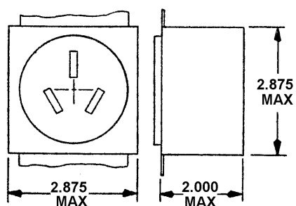
FLUSH MOUNT WC596/36-1
