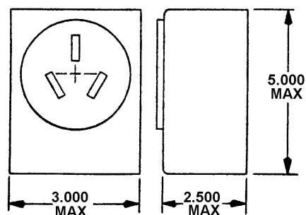
SURFACE MOUNT WC596/36-2
