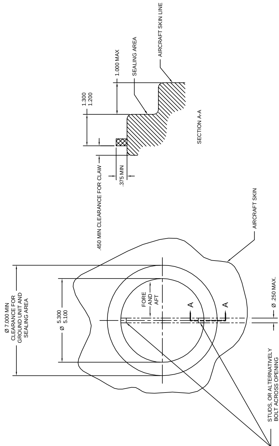
FIGURE 1. Connection, aircraft
