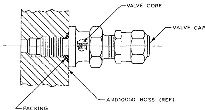
TYPICAL ASSEMBLY
