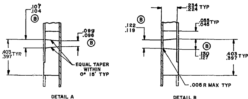
VIEWS OF INSERT POSITIONING GROOVES
