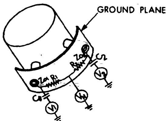
FIGURE 1. Termination assembly.
