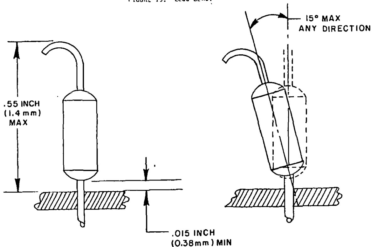
FIGURE 20. Perpendicular part mounting.
