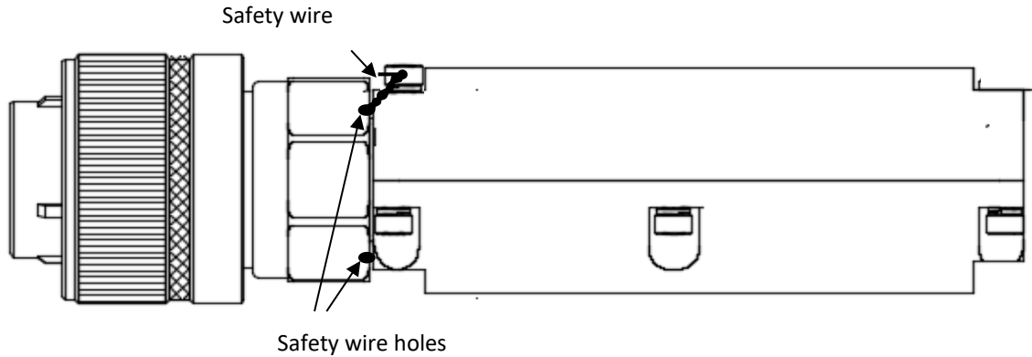
FIGURE 5701-2. Safety wire routing for split backshell coupling nut to shell halves.
