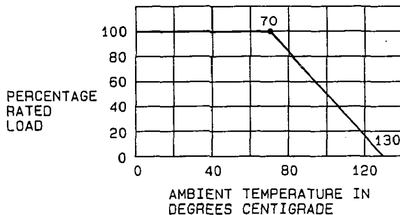
FIGURE 1. Style RCR32 resistor.
