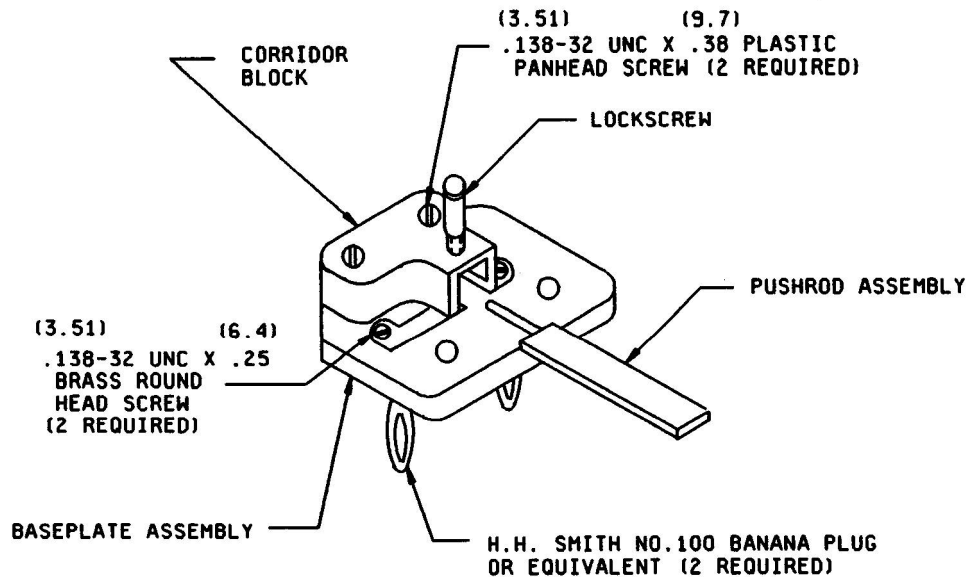
FIGURE 2. Typical chip coil test fixture (TF-250RX-1, or equivalent).
