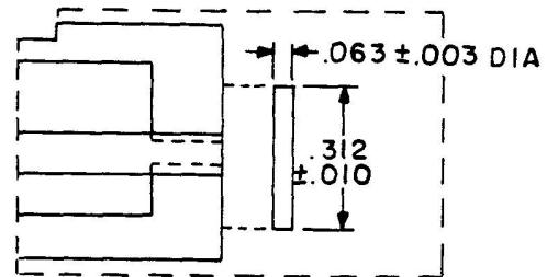
SHORTING BAR LOCATION DETAIL
