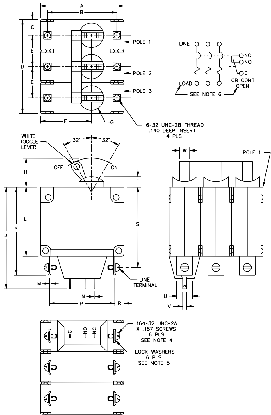
FIGURE 2. Dimensions and configurations (configuration 2).
