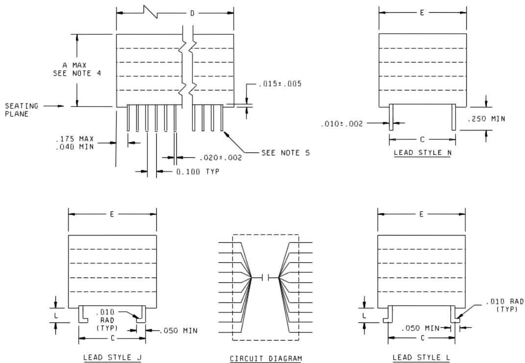
FIGURE 1. Style PS02 capacitors.
