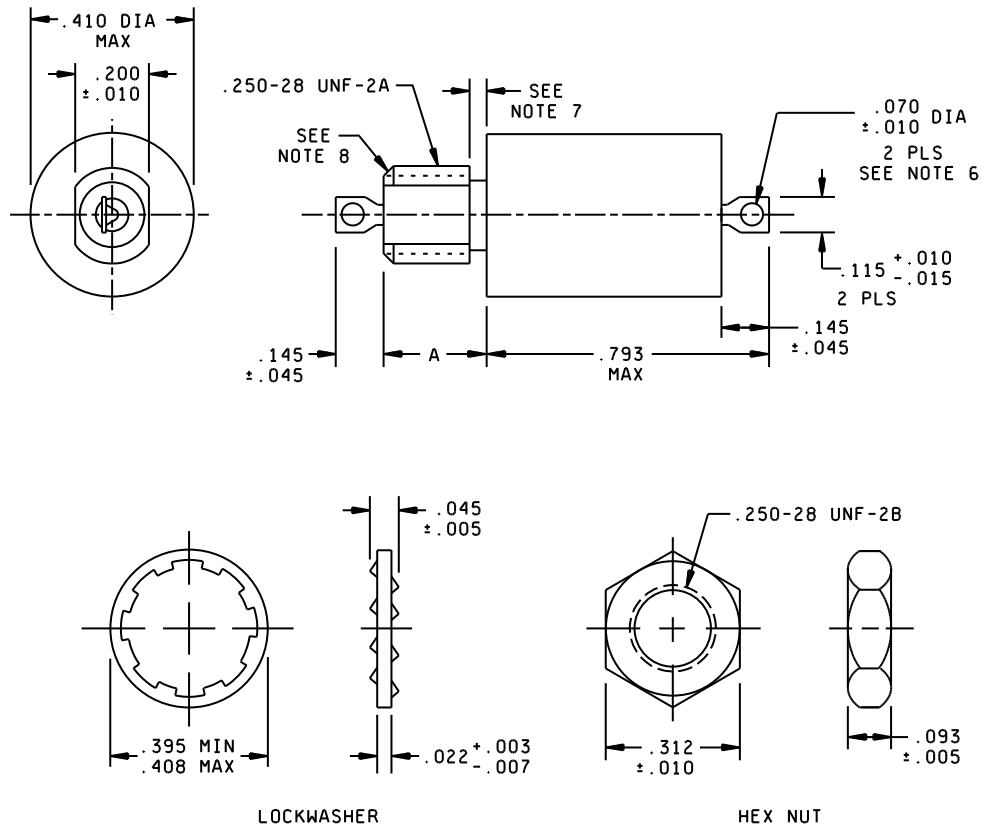
FIGURE 1. Case and hardware dimensions and circuit diagrams.
