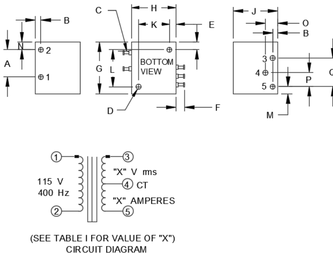
FIGURE 1. Dimensions and configurations.
