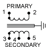
CIRCUIT DIAGRAM "A"
