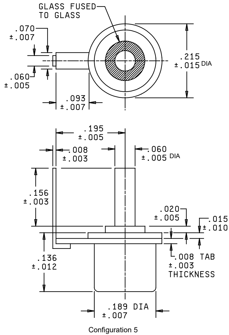
FIGURE 1. Switches - Continued.
