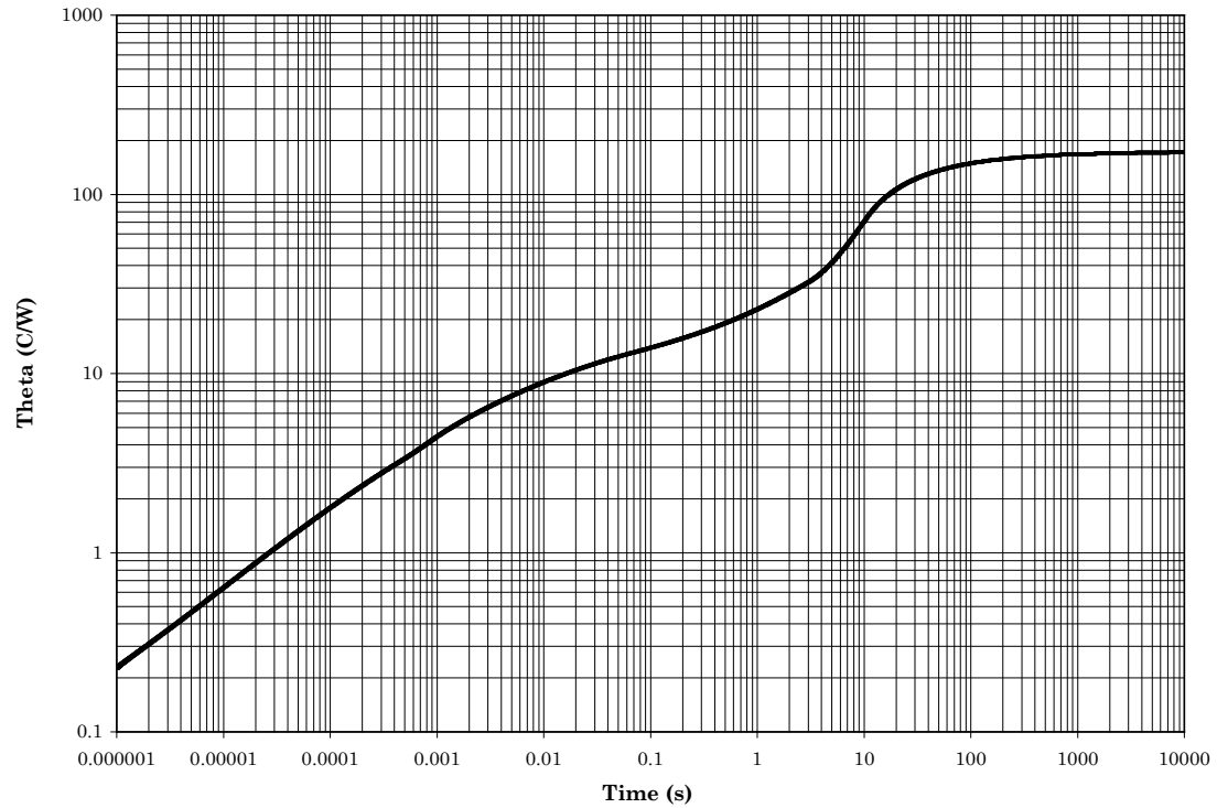
FIGURE 8. Thermal impedance graph ( R_{\theta JA} ) for 2N3506, 2N3506A, 2N3506L, 2N3506AL, 2N3506U4, 2N3506AU4, 2N3507, 2N3507A, 2N3507L, 2N3507AL, 2N3507U4, and 2N3507AU4.
