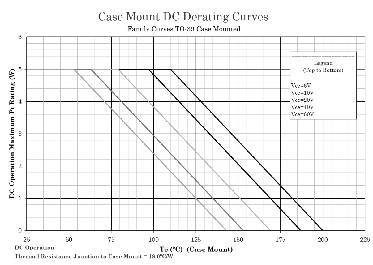
FIGURE 7. Temperature-power derating for 2N3506, 2N3506A, 2N3506L, 2N3506AL, 2N3507, 2N3507A, 2N3507L, and 2N3507AL.
