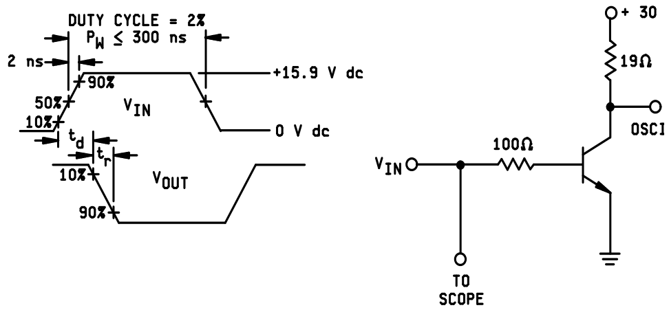
FIGURE 11. Equivalent circuit for measuring delay and rise times.
