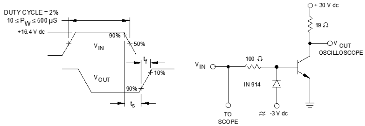
* FIGURE 12. Equivalent circuit for measuring storage and fall times.
