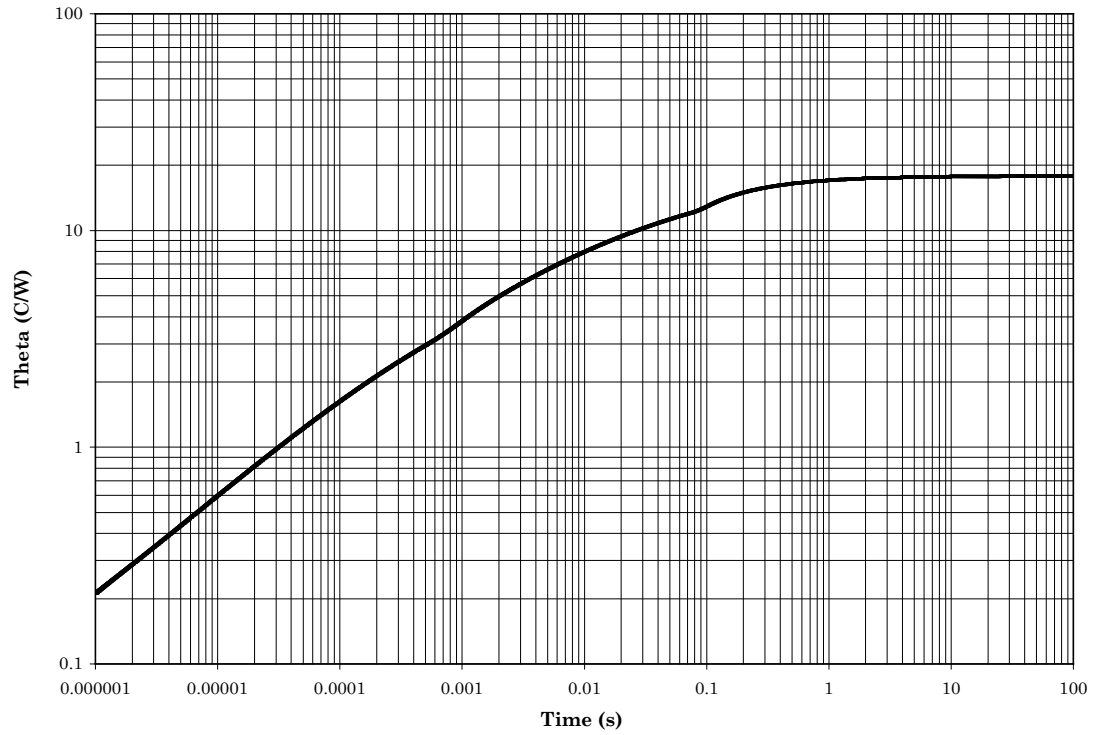
FIGURE 9. Thermal impedance graph ( R_{\theta JC} ) for 2N3506, 2N3506A, 2N3506L, 2N3506AL, 2N3507, 2N3507A, 2N3507L, and 2N3507AL.
