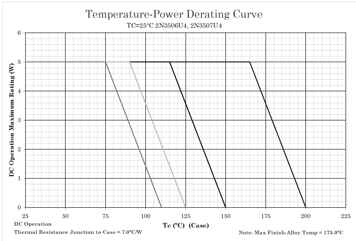
FIGURE 6. Temperature-power derating for 2N3506U4, 2N3506AU4, 2N3507U4, and 2N3507AU4.
