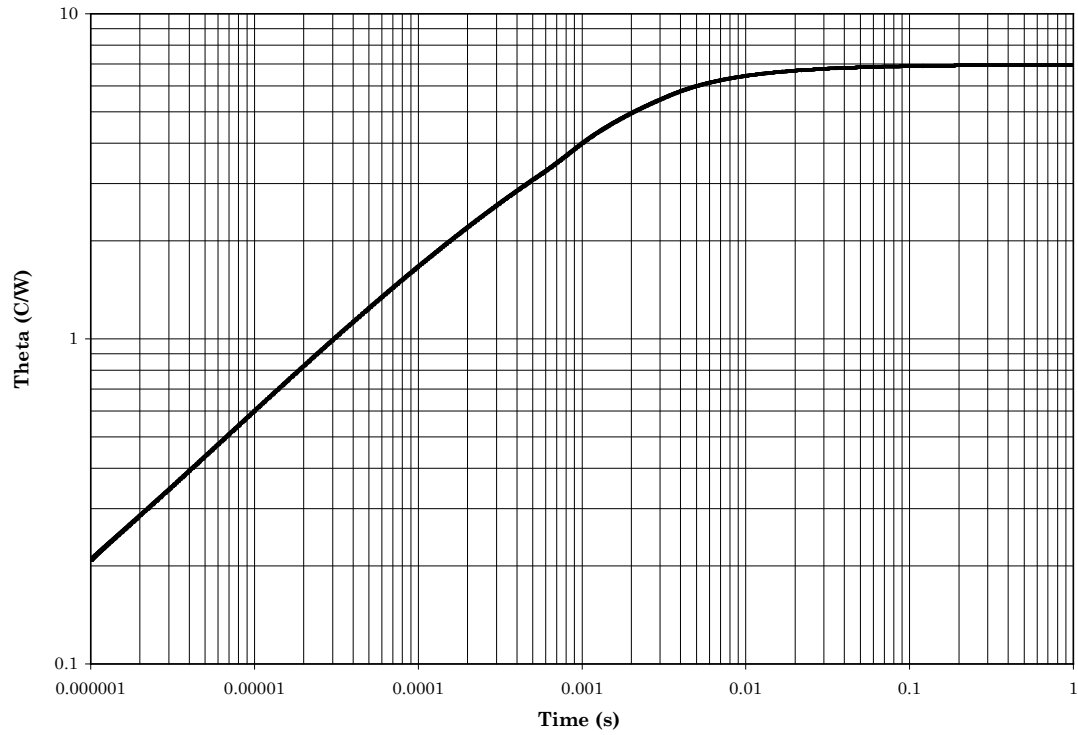
FIGURE 10. Thermal impedance graph ( R_{\theta JC} ) for 2N3506U4, 2N3506AU4, 2N3507U4, and 2N3507AU4.
