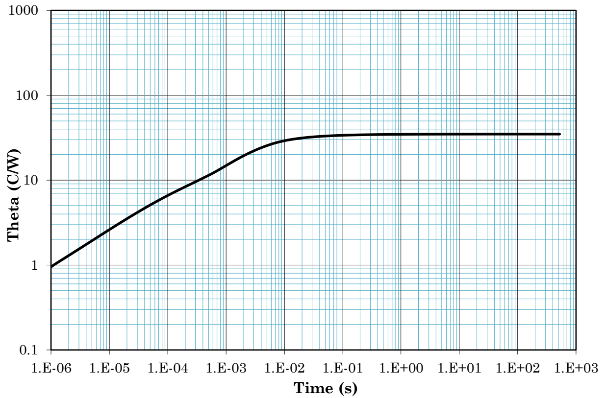
FIGURE 9a. Thermal impedance graph ( R_{\theta JC} ) for Kovar 2N3506, 2N3506A, 2N3506L, 2N3506AL, 2N3507, 2N3507A, 2N3507L, and 2N3507AL.
