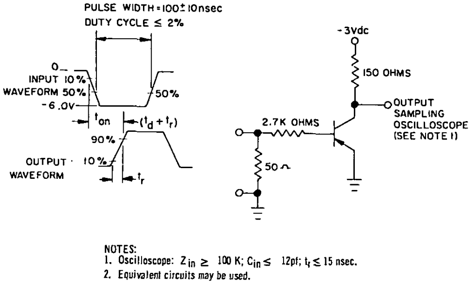
FIGURE 2. Rise switching-time ( t_r ) test circuit.
