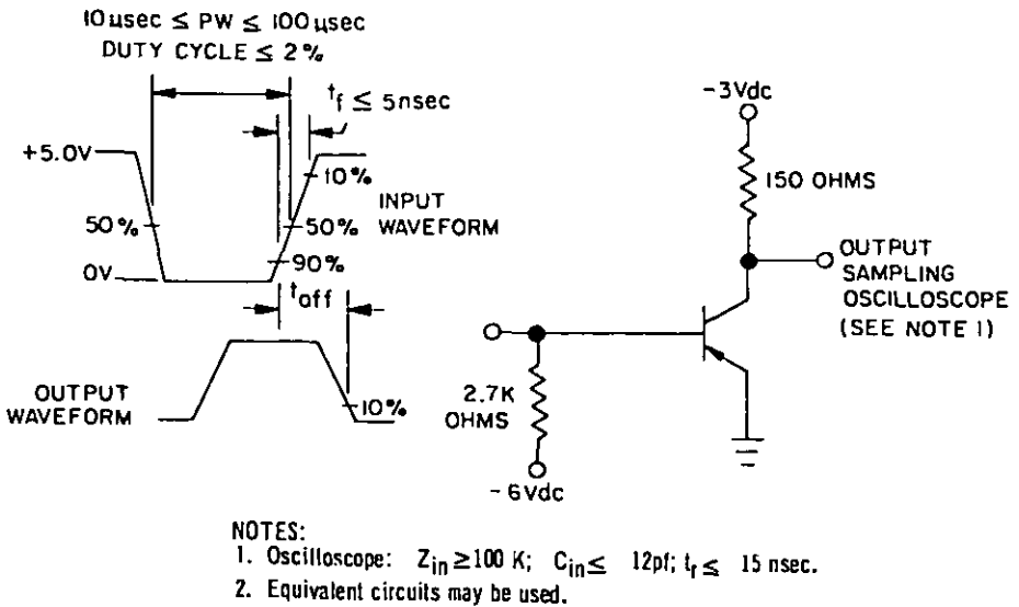
FIGURE 3. Turn-off switching-time ( t_s and t_f ) test circuit.
