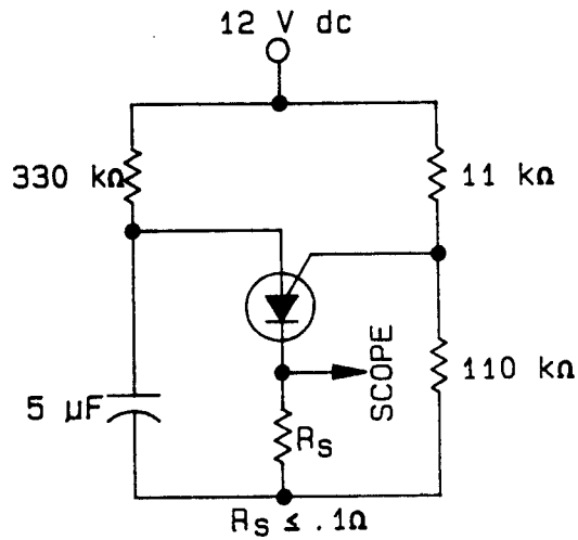
FIGURE 12. Capacitive discharge energy test circuit.
