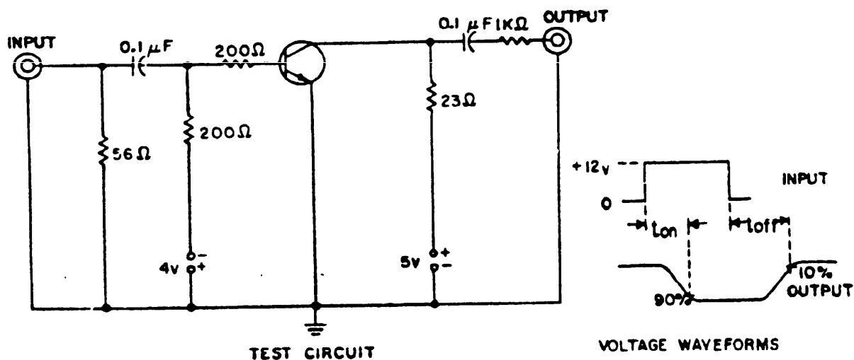
FIGURE 3. Charge storage time ( t_s ) test circuit.
