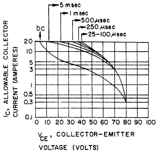
FIGURE 3. Pulse safe-area control curve for transistor type 2N2079A.
