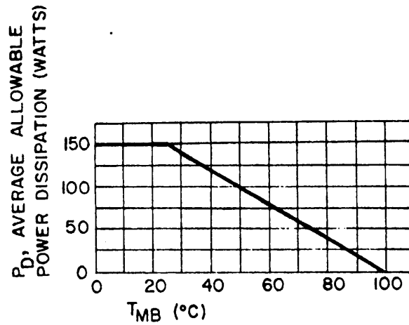
FIGURE 2. Power-temperature derating curve.
