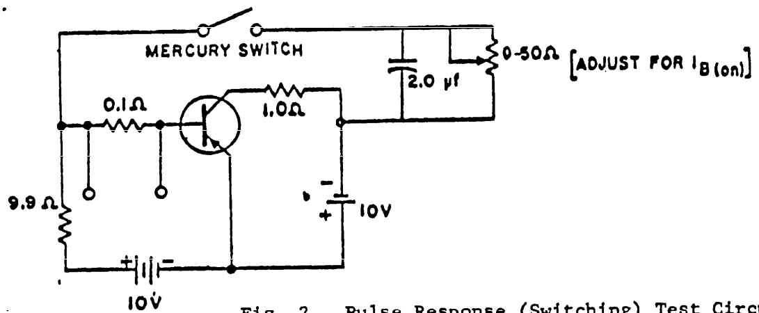
Fig. 2. Pulse Response (Switching) Test Circuit.
