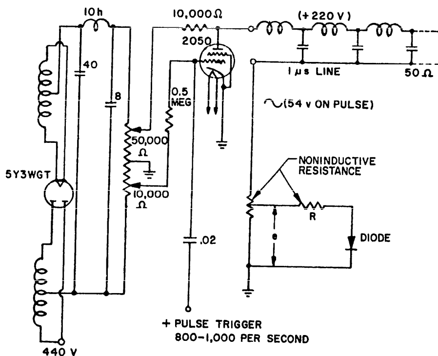
FIGURE 2. Pulse circuit for test burnout.
