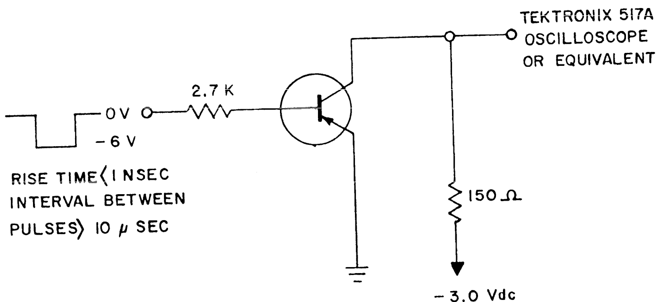
FIGURE 3. Pulse rise-time test circuit.
