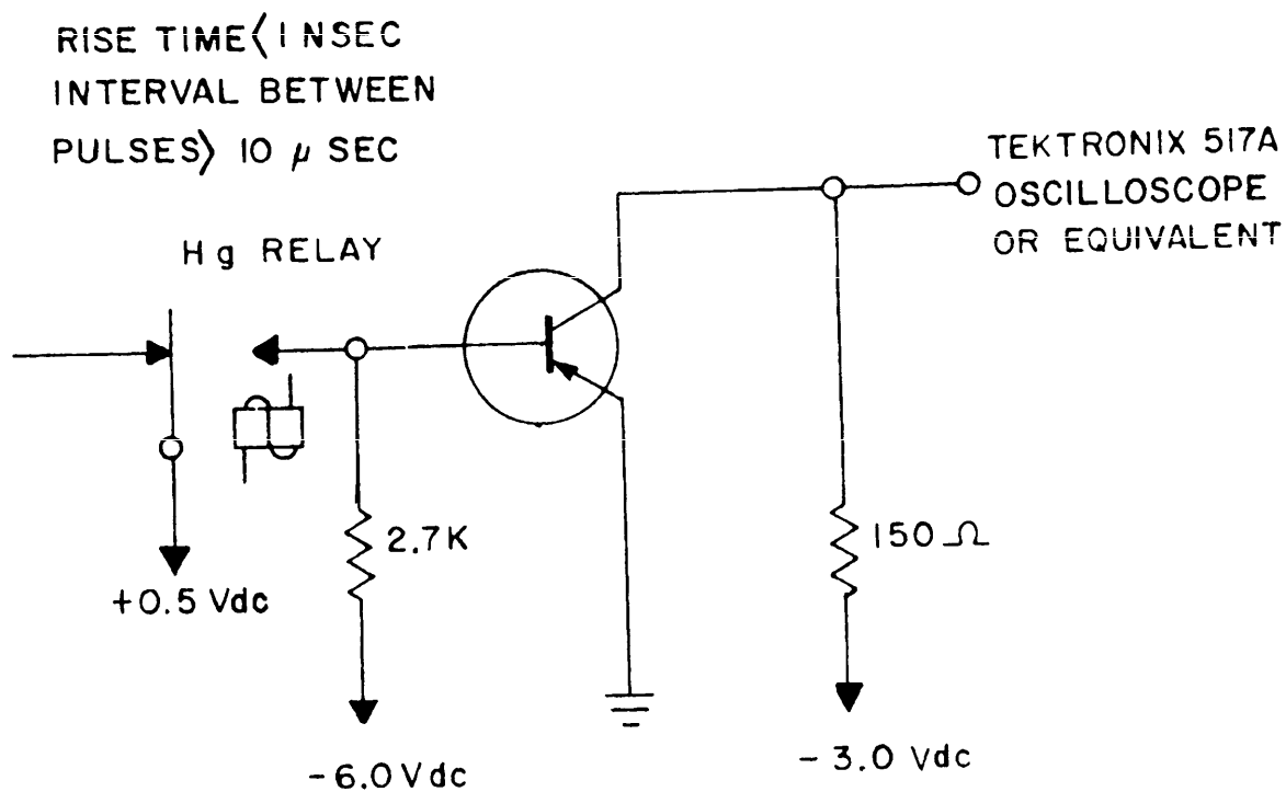
FIGURE 4. Pulse storage and fall-time test circuit.
