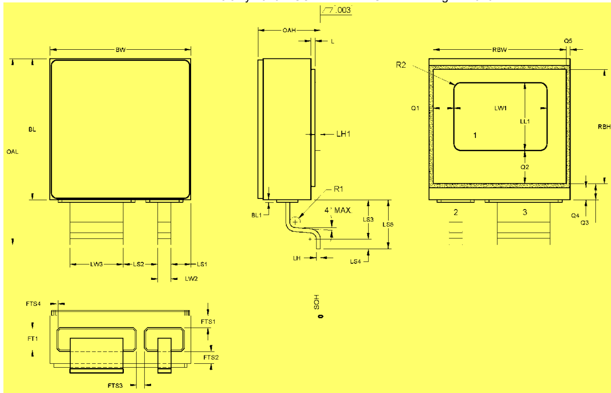
FIGURE 1. Physical dimensions, U2A surface mount (2N7663U2A).
