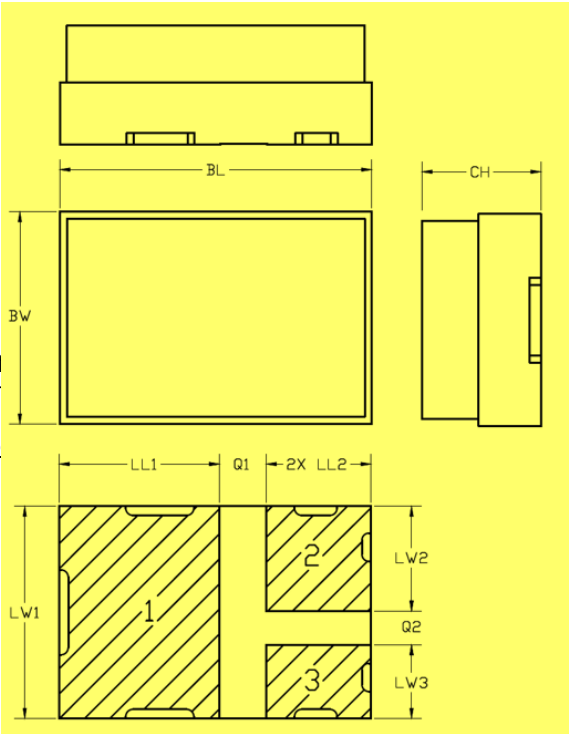
* FIGURE 1. Dimensions and confi
