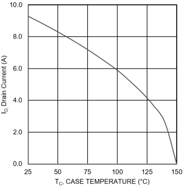
FIGURE 3. Maximum drain current versus case temperature graphs.
