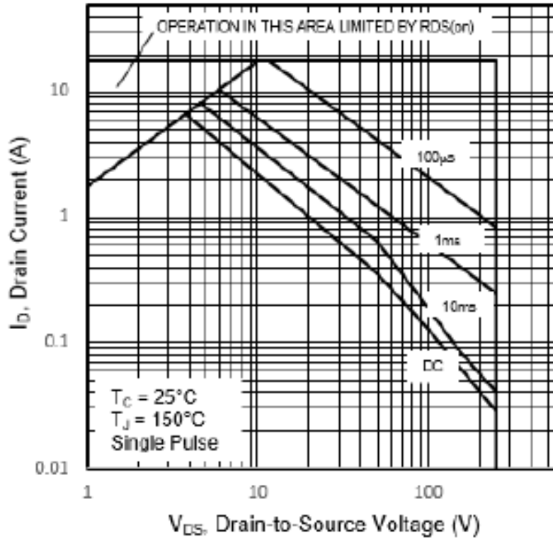
FIGURE 4. Safe operating area graphs.
