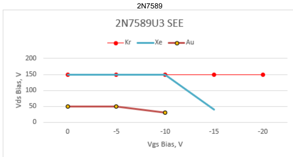
FIGURE 8 9. Typical SEE safe operating area response (CAGE 43611).
