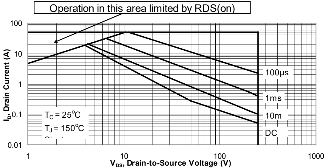
FIGURE 6 7. Safe operating area graph – Continued.
