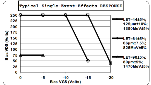
FIGURE 7 8. Typical SEE safe operating area graphs (CAGE 69210).
