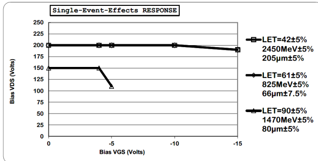
FIGURE 7 8. Typical SEE safe operating area graphs (CAGE 69210).
