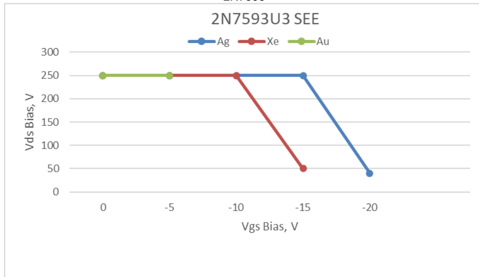
FIGURE 40 11. Typical SEE safe operating area response (CAGE 43611).
