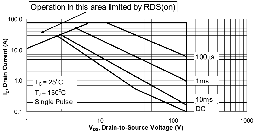
FIGURE 6 7. Safe operating area graph.
