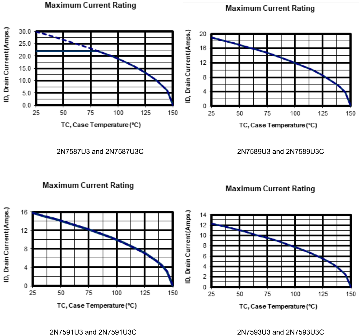
FIGURE 5 6. Maximum drain current versus case temperature graphs.
