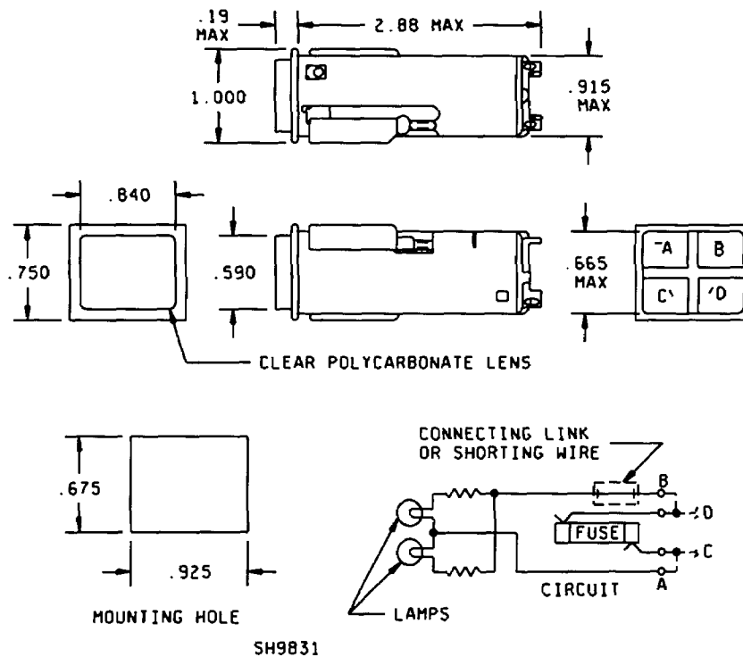
FIGURE 1. Type FHL49U fuseholder.
