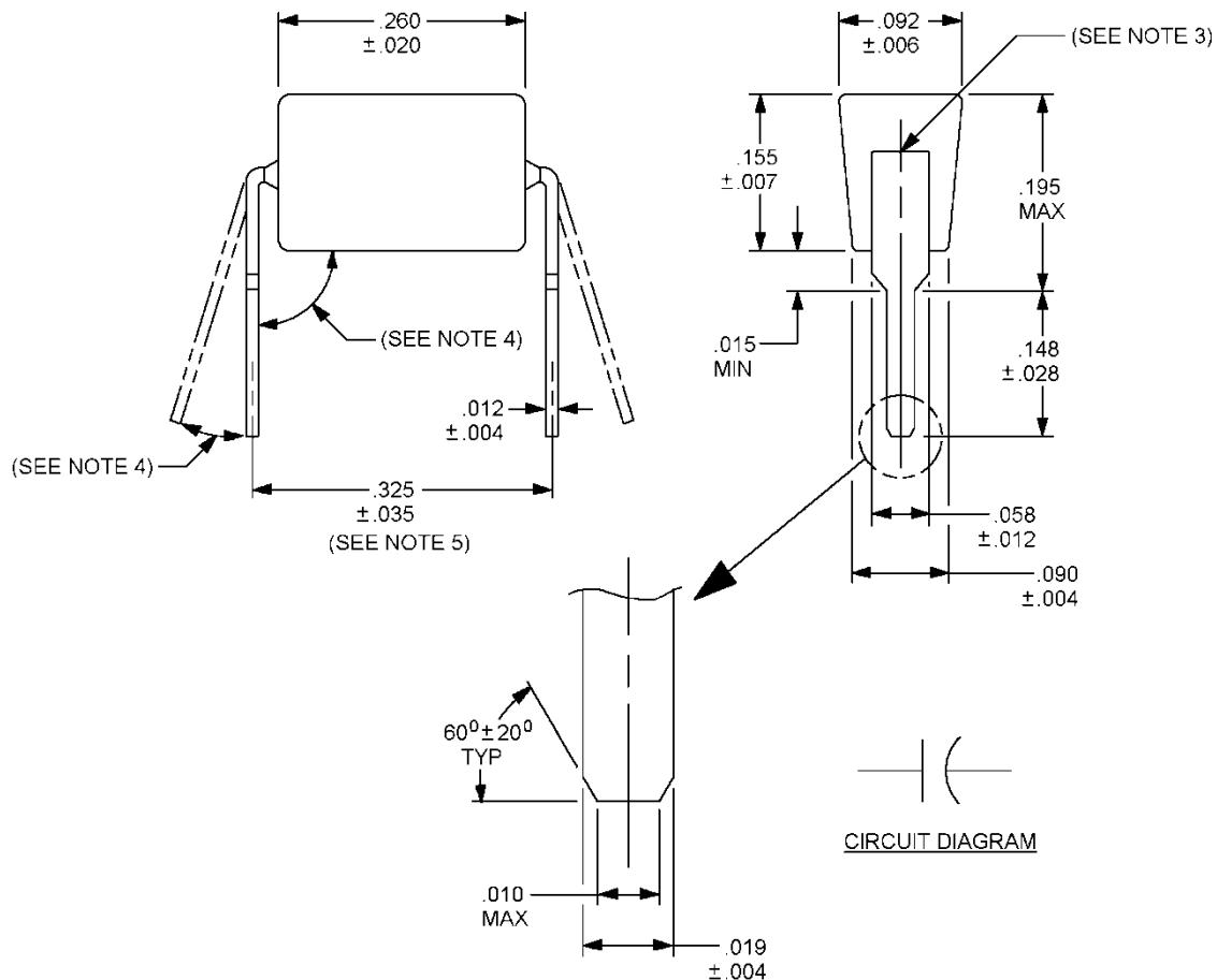
FIGURE 1. Style CKS23 capacitors.
