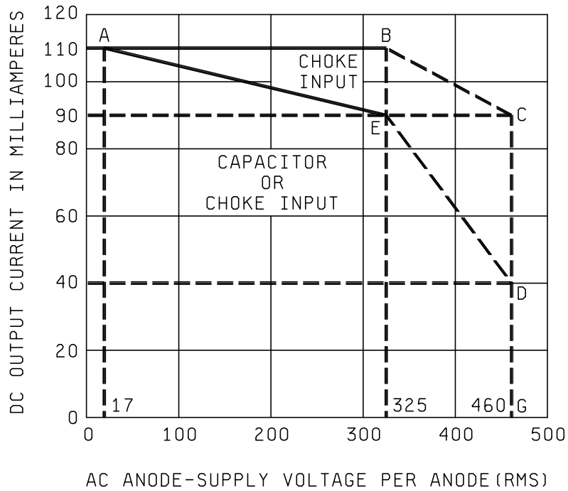
FIGURE 2. Rating chart I absolute maximum ratings.
