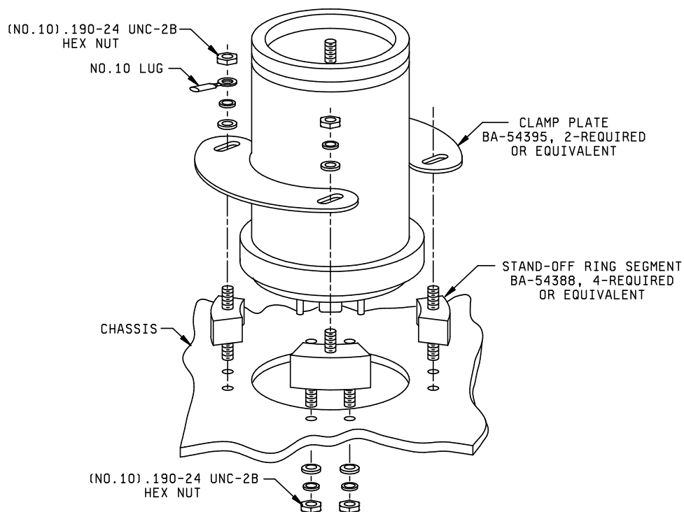
FIGURE 3. MT-4 tube mounting assembly.
