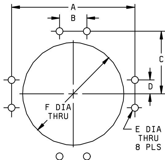
FIGURE 2. Mounting hole dimensions.
