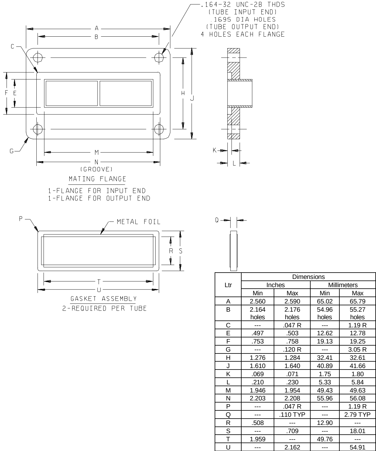
FIGURE 2. Mating flange and gasket assembly.
