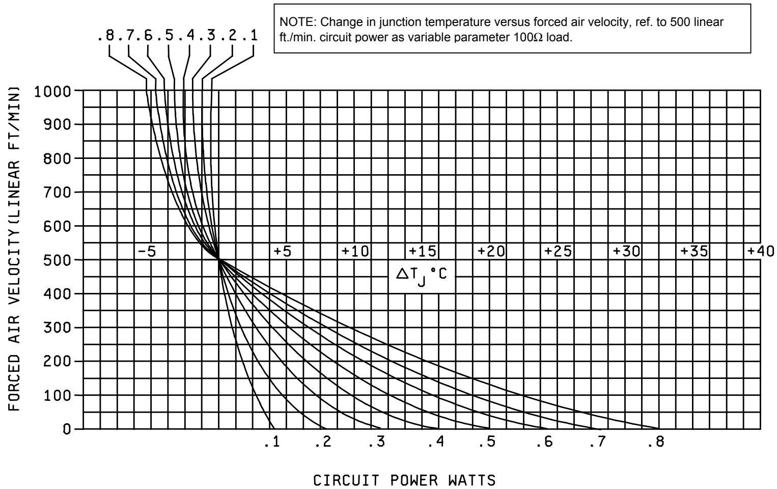
FIGURE 15. Junction temperature versus air velocity case F.
