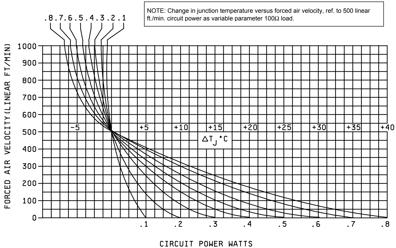
FIGURE 14. Junction temperature versus air velocity case E.
