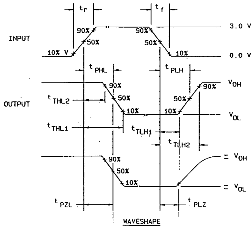
FIGURE 2. Switching time test circuit and waveforms.
