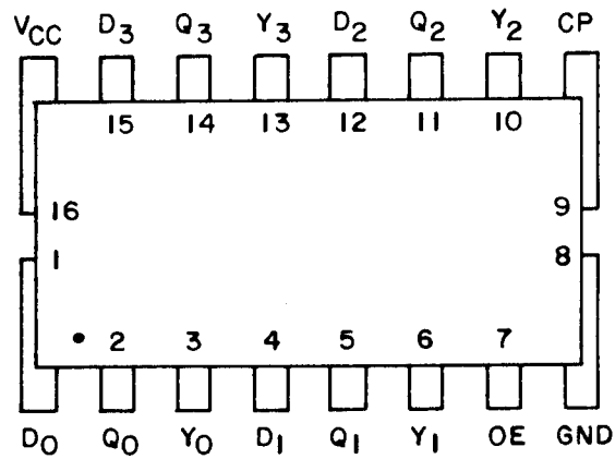
FIGURE 1. Terminal connections.
