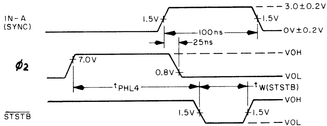
Waveform B
