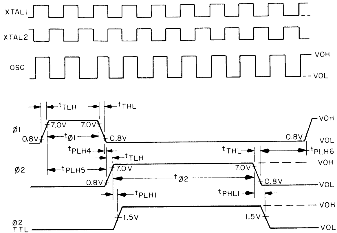
Waveform A
