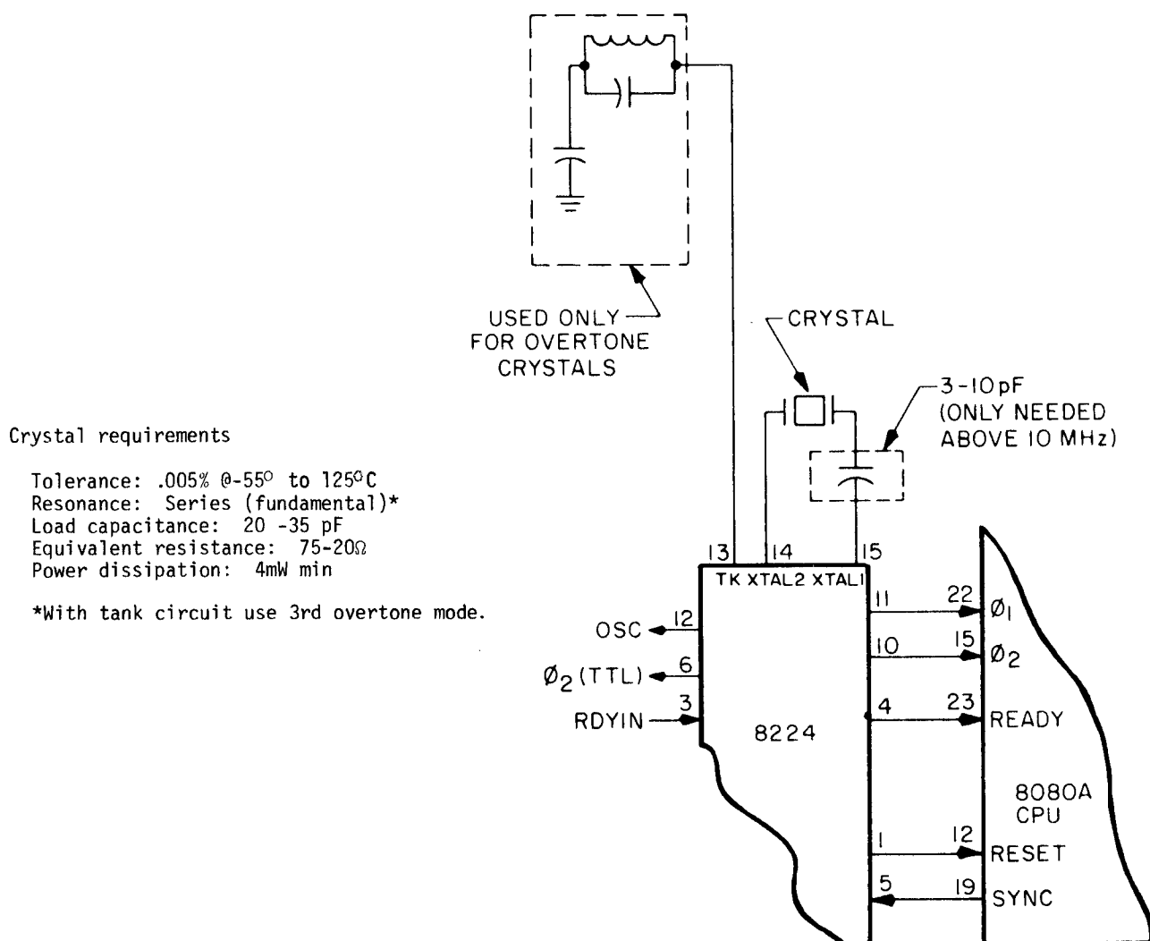
FIGURE 3. Crystal input requirements.
