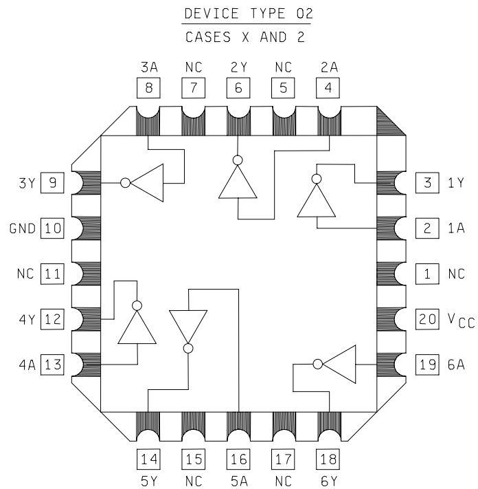
FIGURE 1. Terminal connections and logic diagrams - Continued.
