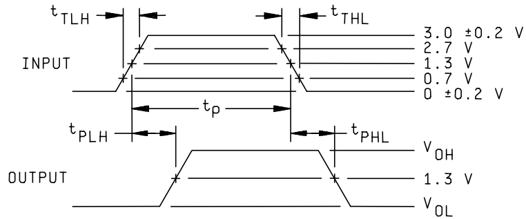
VOLTAGE WAVEFORMS
