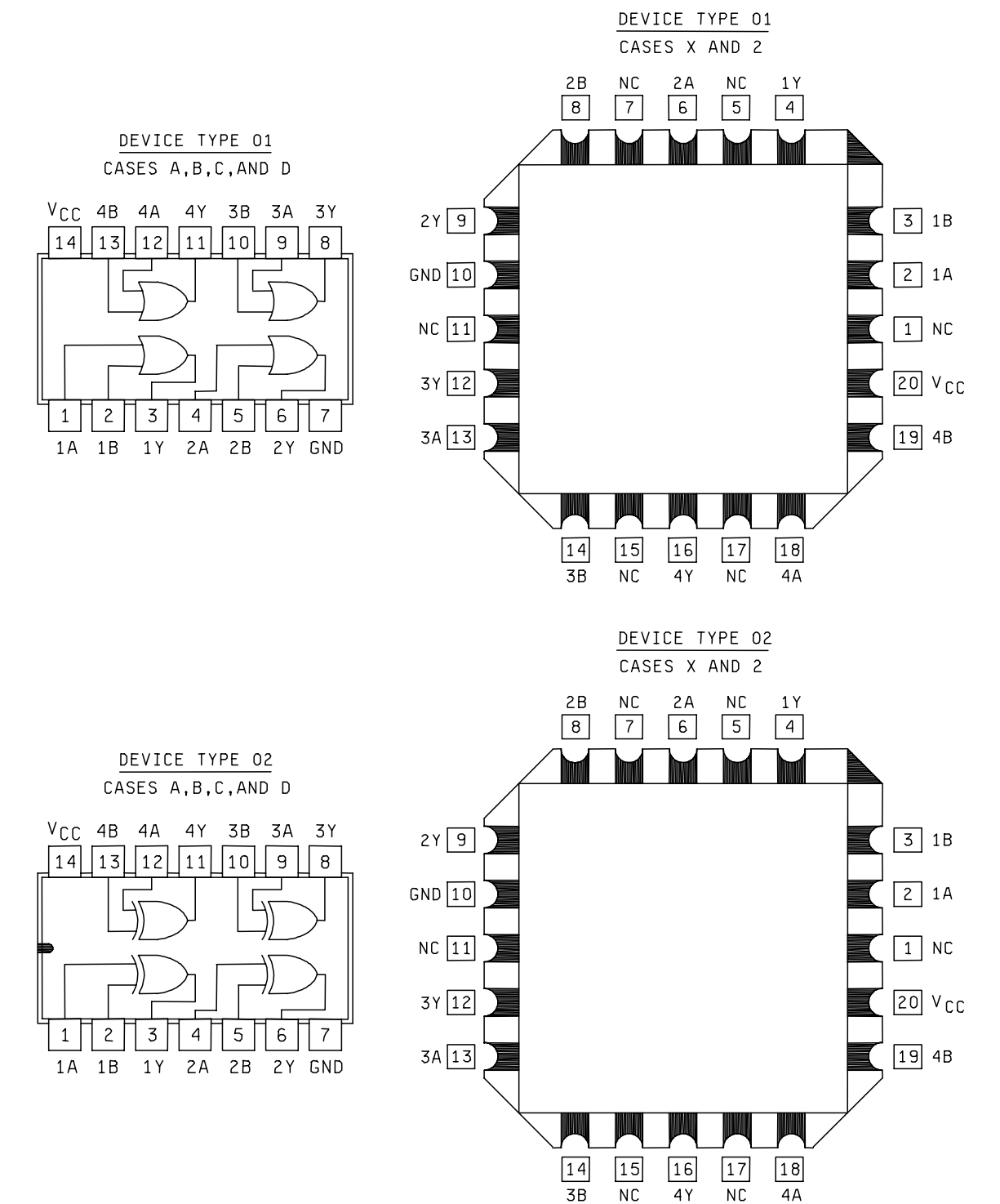
FIGURE 1. Terminal connections and logic diagrams.
