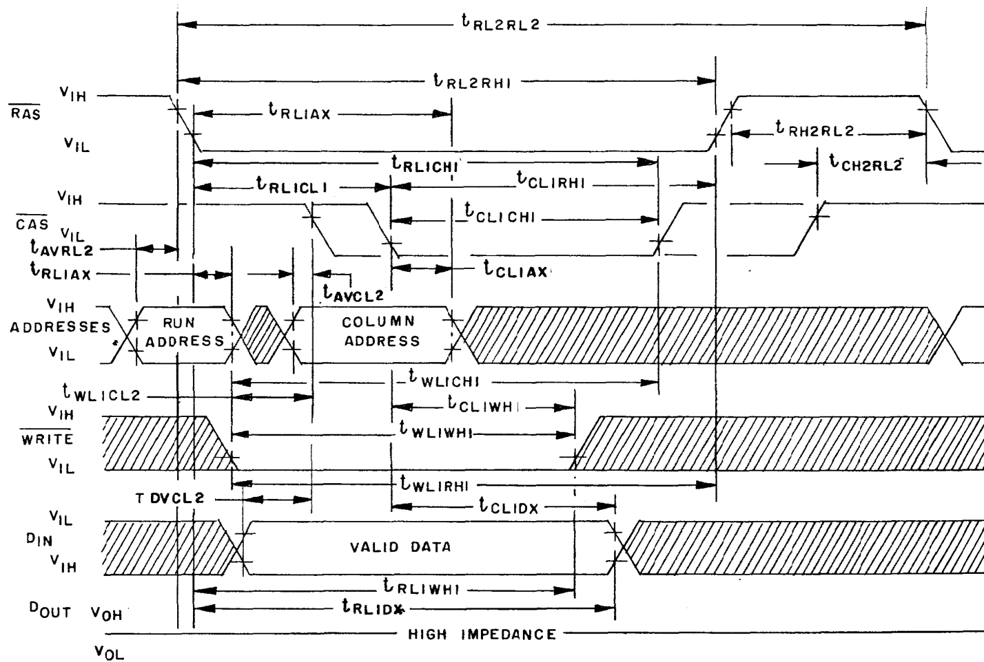
FIGURE 8. Write cycle waveforms.
