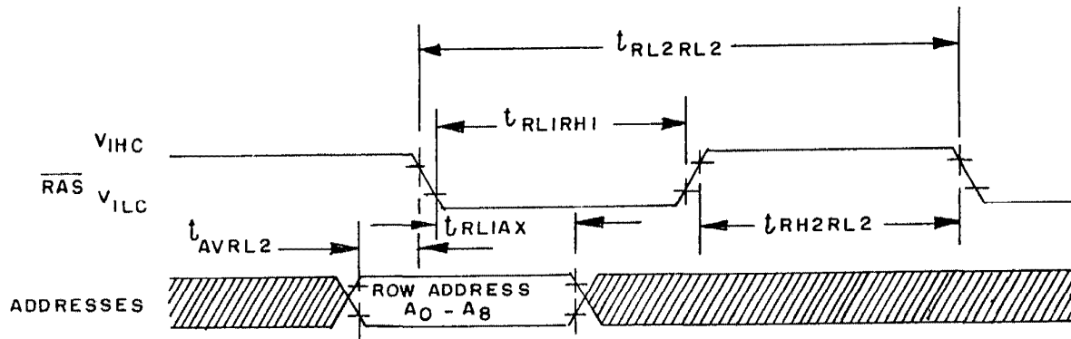
FIGURE 10. RAS-only refresh cycle waveforms.
