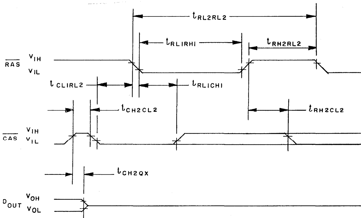
FIGURE 11. CAS before RAS refresh cycle waveforms.
