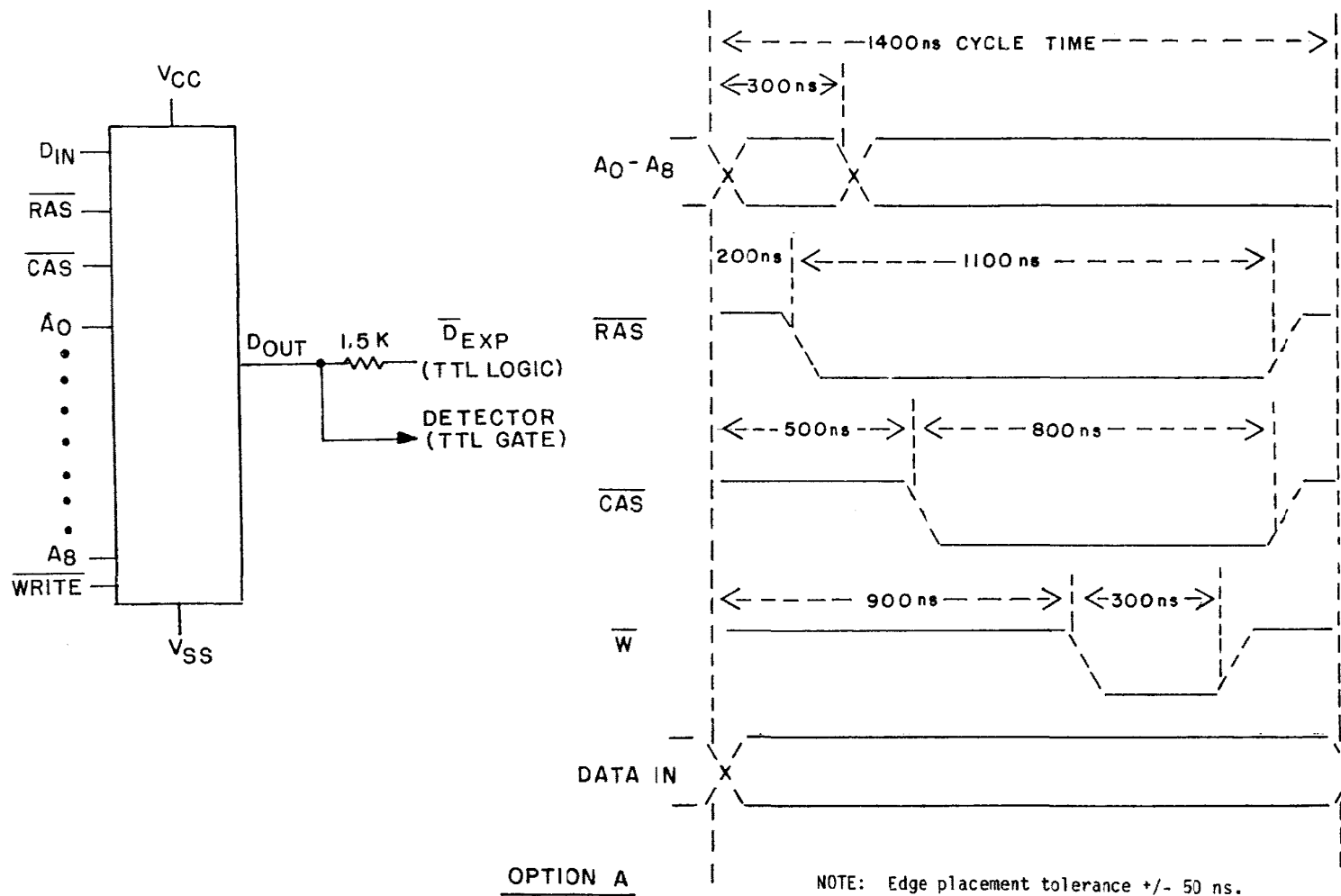
FIGURE 5. Alternative burn-in and steady-state life test circuits.- Continued.
