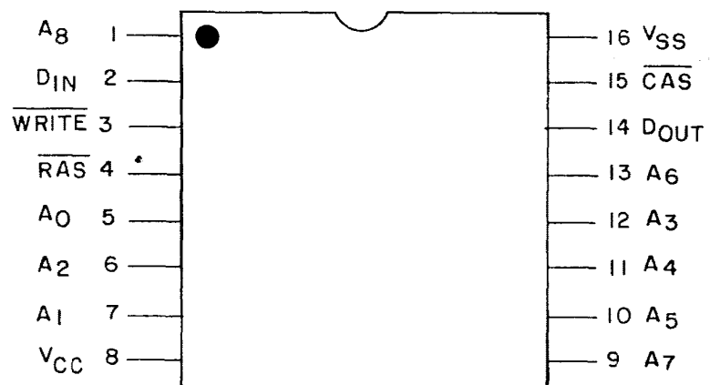
Case E - Top view
