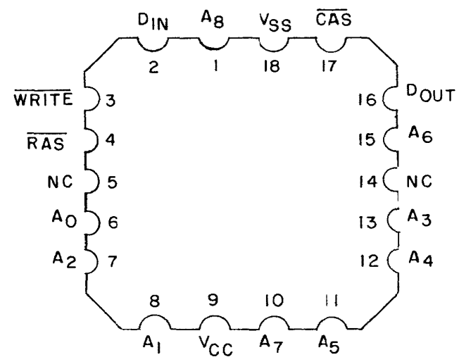
Case X - Top view
