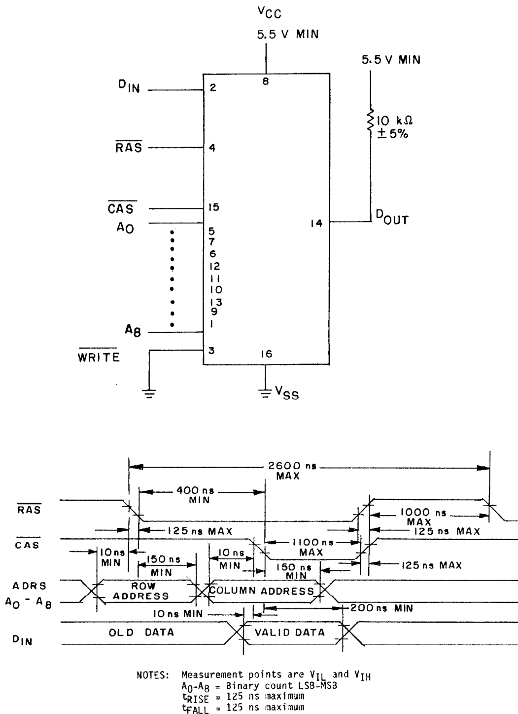
FIGURE 5. Burn-in and steady state life test circuit.
