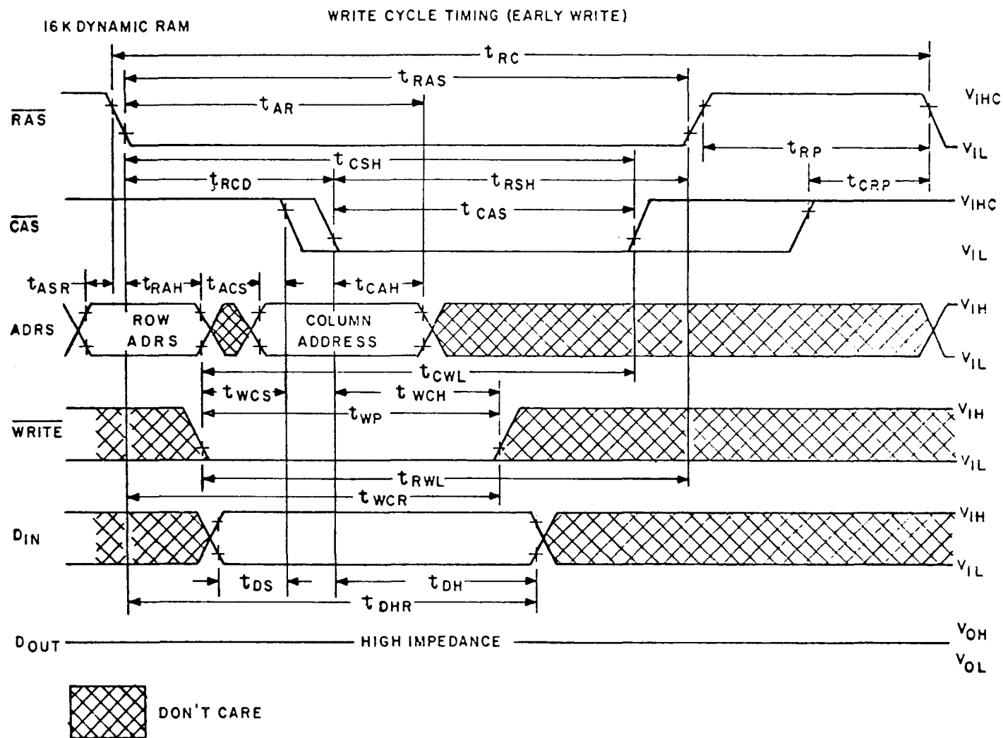
FIGURE 8. Write cycle waveforms.
