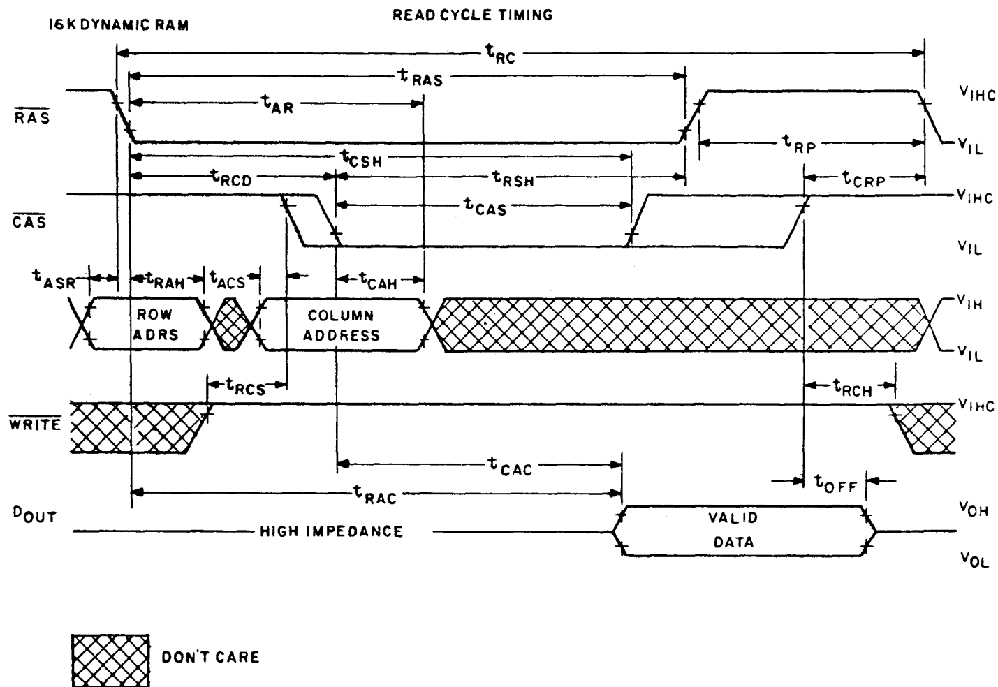
FIGURE 7. Read cycle waveforms.
