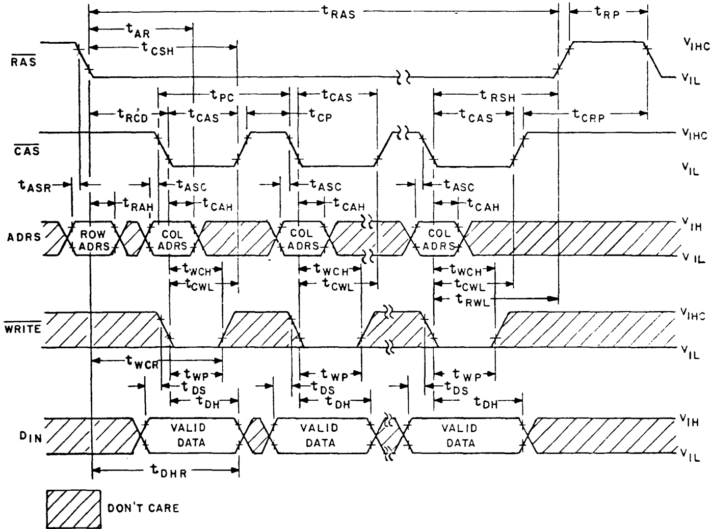
FIGURE 12. Page mode write cycle waveforms.
