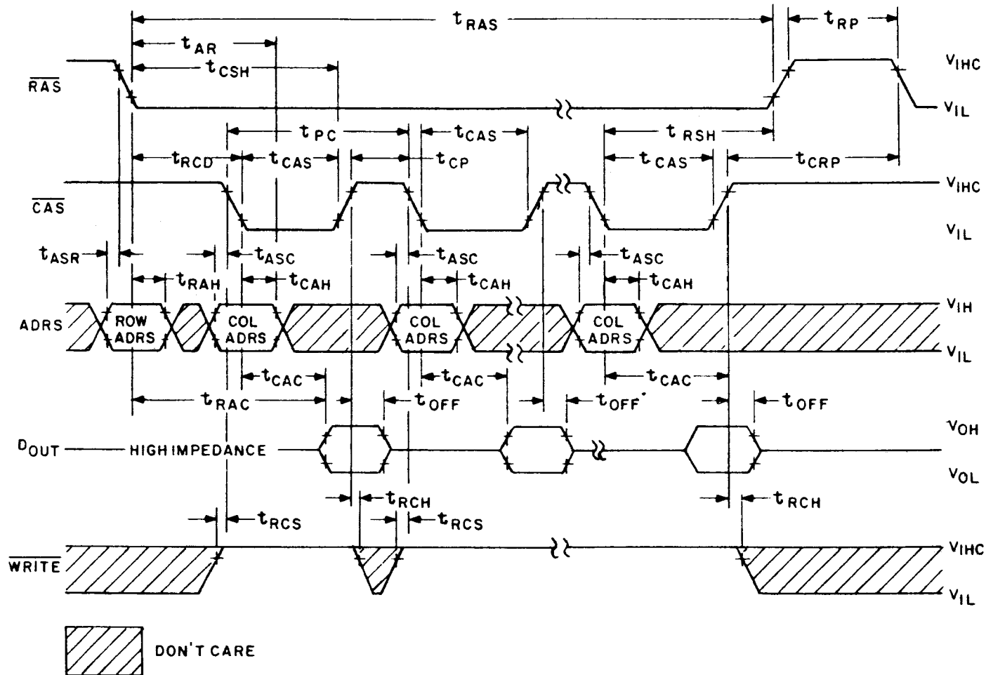
FIGURE 11. Page mode read cycle waveforms.
