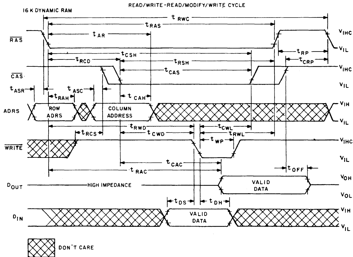
FIGURE 9. Read/write, read modify write cycle waveforms.
