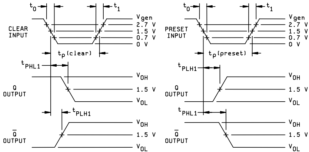
VOLTAGE WAVEFORMS
