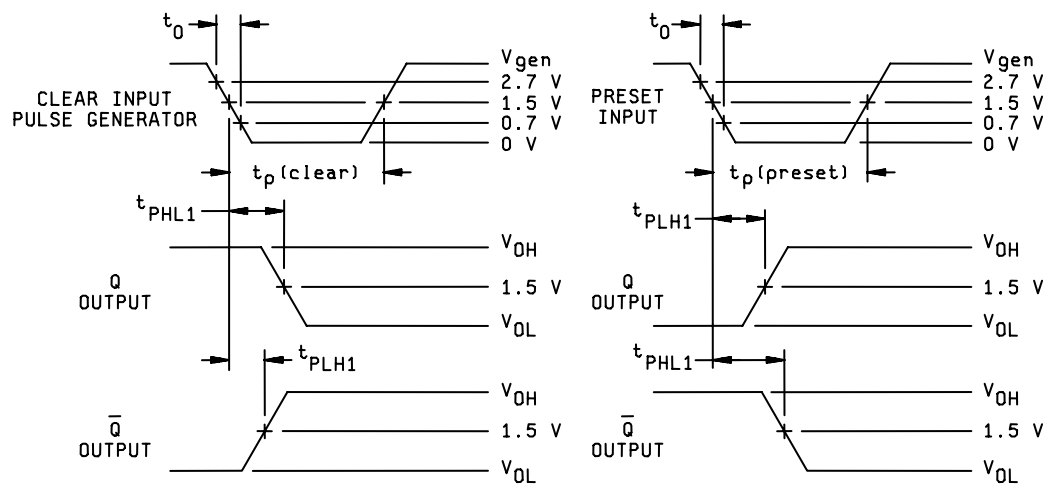
VOLTAGE WAVEFORMS
