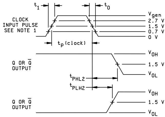
VOLTAGE WAVEFORMS
