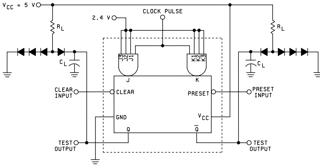
TEST CIRCUIT
