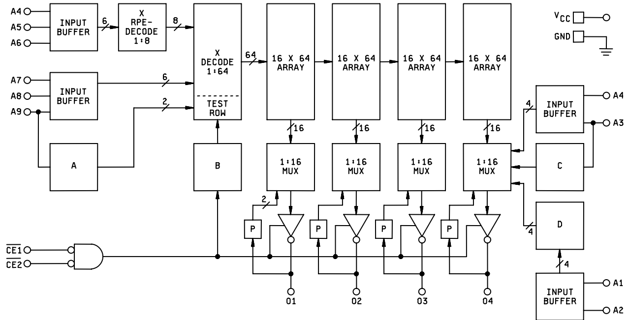
CIRCUIT C
