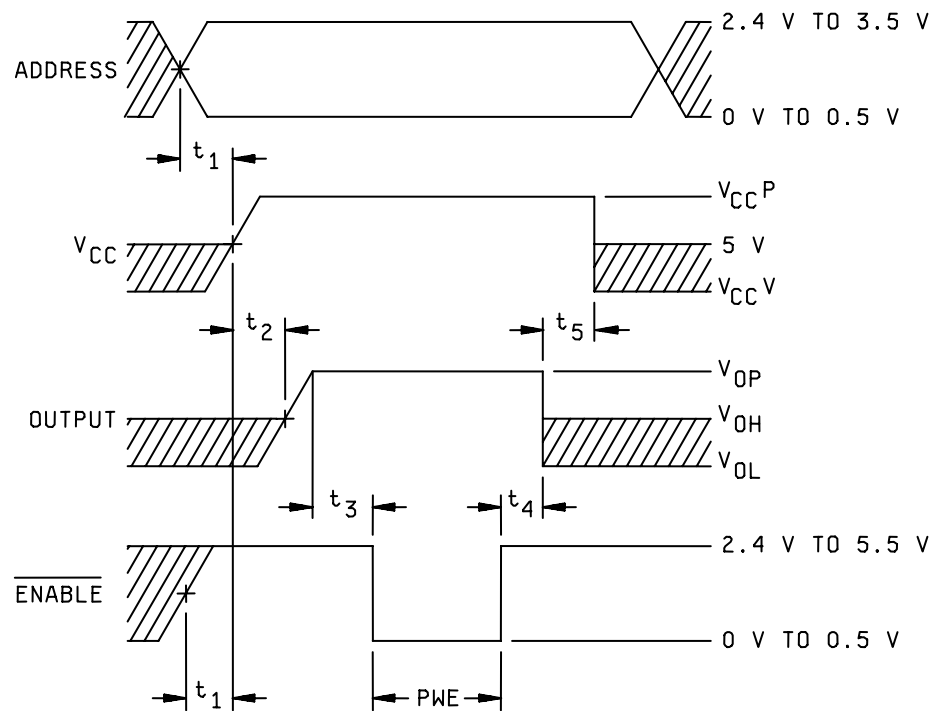
FIGURE 6D Programming voltage waveforms during programming for circuit D.
