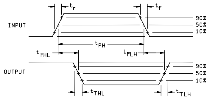
DYNAMIC TEST WAVEFORMS
